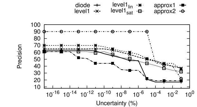
Fig. 4: Crossover Precision for Different Devices
